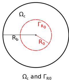
\Omega_c and \Gamma_{R_0}
