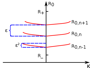
Figure 1.3: The admissible radii \{R_{0,n}\} graphed versus \kappa for fixed \varepsilon . The gaps between successive radii are \mathcal{O}(\varepsilon) while the variation in R_{0,n} with \kappa is \mathcal{O}(\varepsilon^2) .
