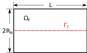
\Omega_f and \Gamma_f
